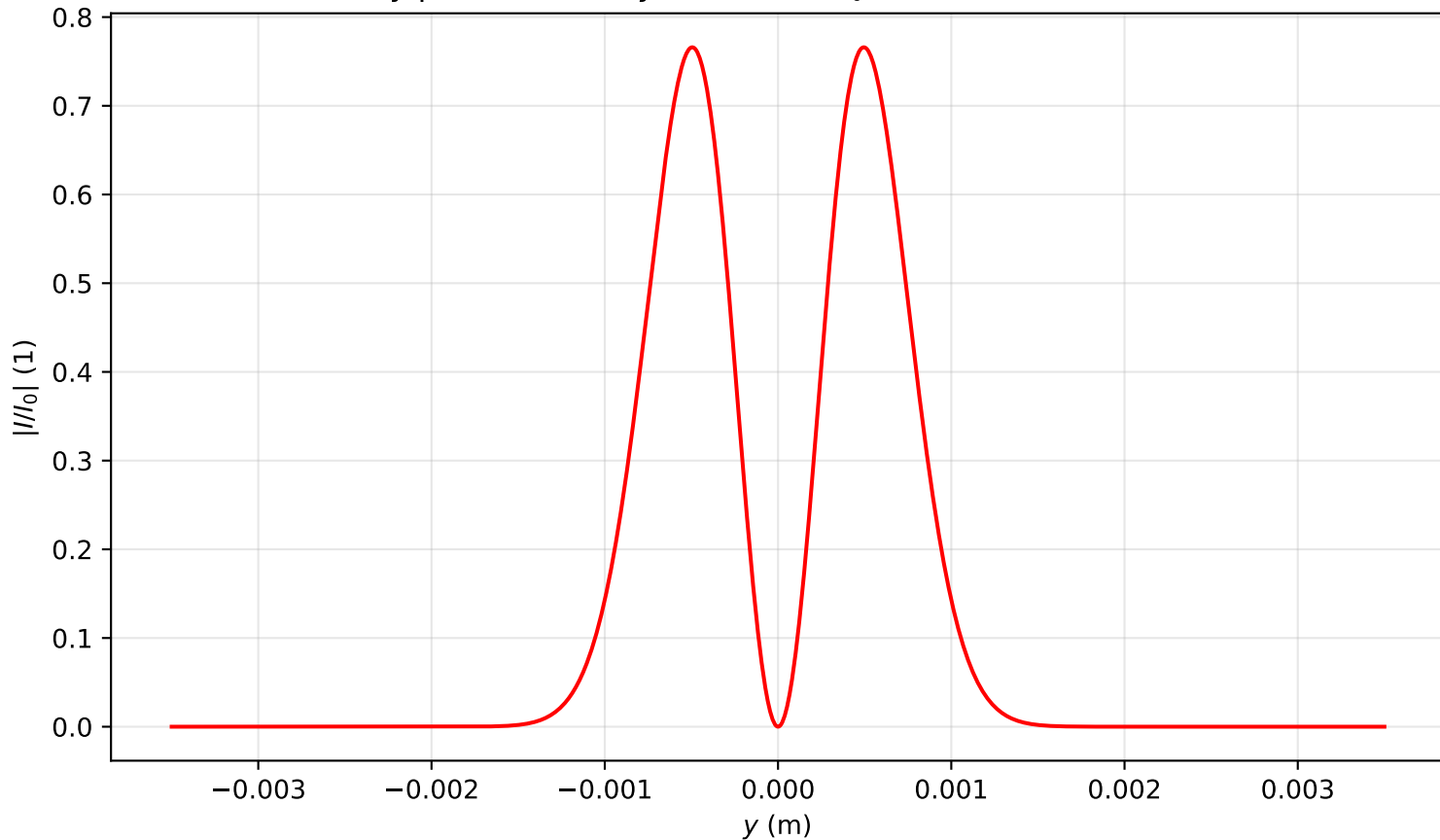
Intensity profile I(x=0, y, z=0.080)/I_0 , P_{in}=1.0P_{cr} , artificial time
